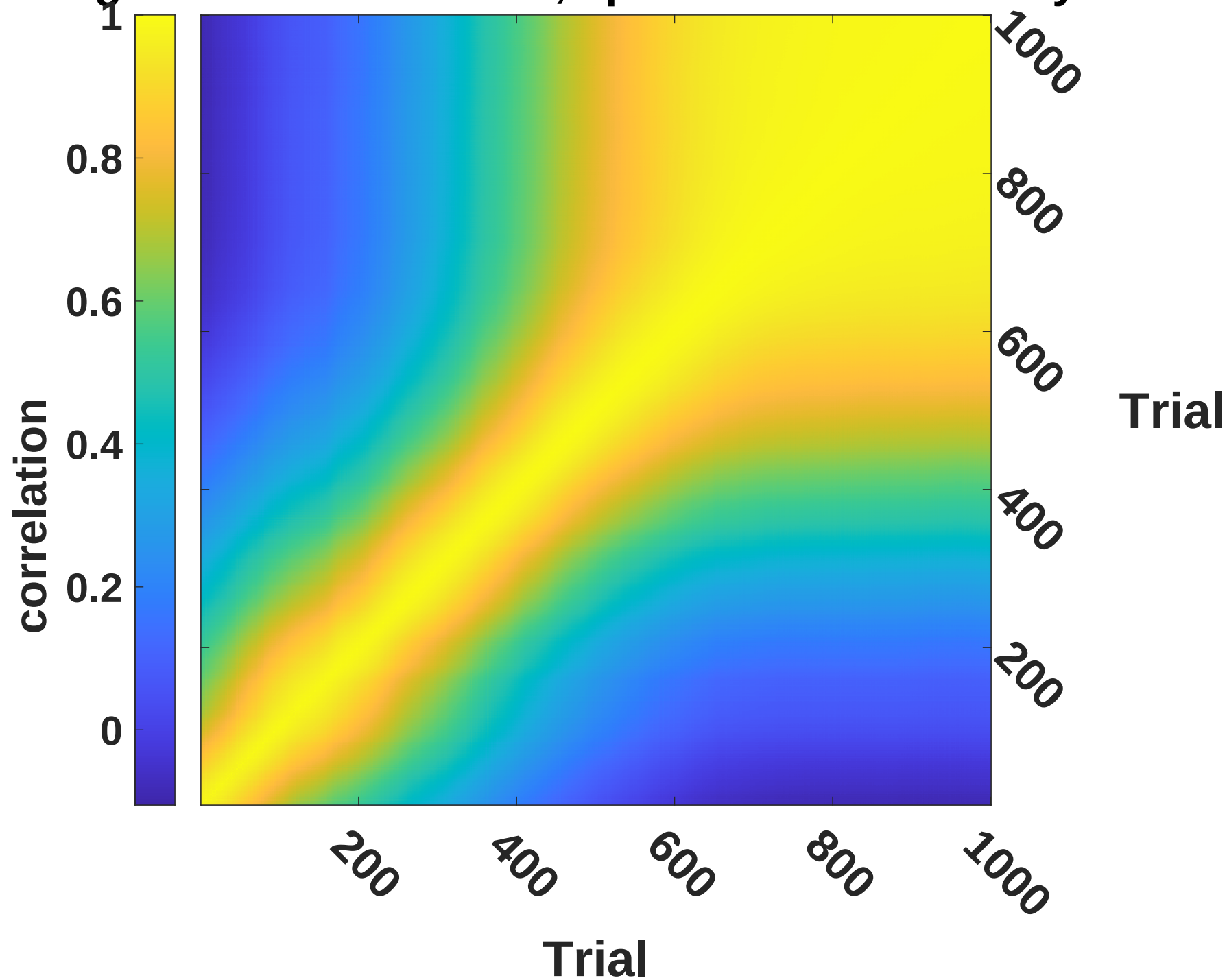
Averaged on 3 Simulations, spike counts Similarity Matrix
